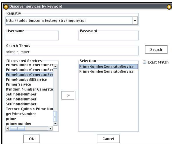
Figure 2. Service Discovery in SQRM
