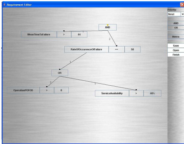
Figure 3. Requirement Creation in SQRM
