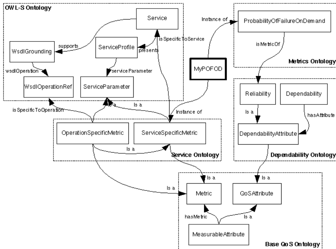
Figure 1. QoS Ont Structure
