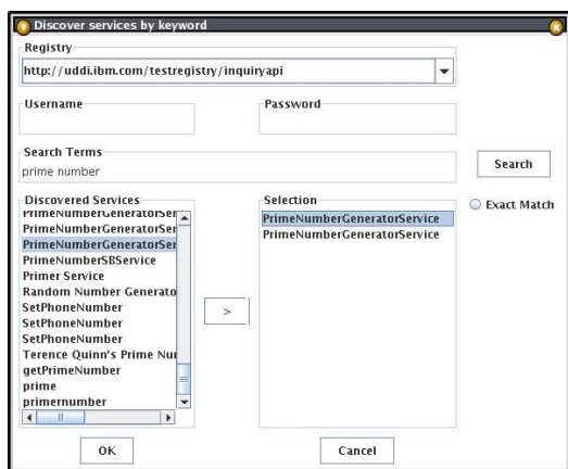
Figure 2. Service Discovery in SQRM
