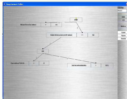
Figure 3. Requirement Creation in SQRM
